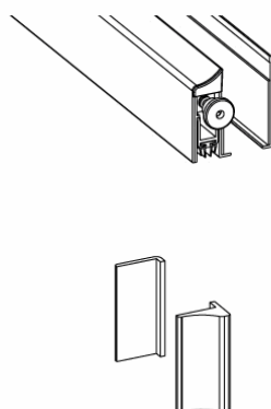
PLUNGER TYPE
